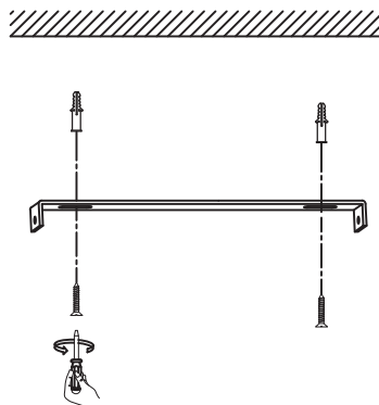
Tie up screws to make it stable
