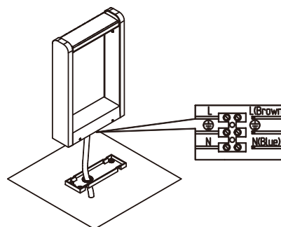
Connect the wires
