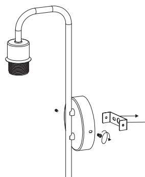
4. Fix the mounting bar and canopy with screw
