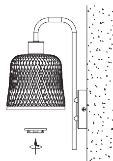
6. Fasten the lamp shade with the plastic ring
