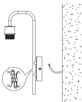
3. Brown (Active) connect it with marked "L" Blue (Neutral) connect it with marked "N" Green & yellow connect it with marked "↓"
