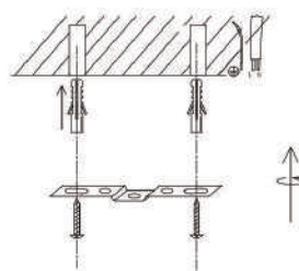
2. Drill holes, apply plastic anchors & screws
